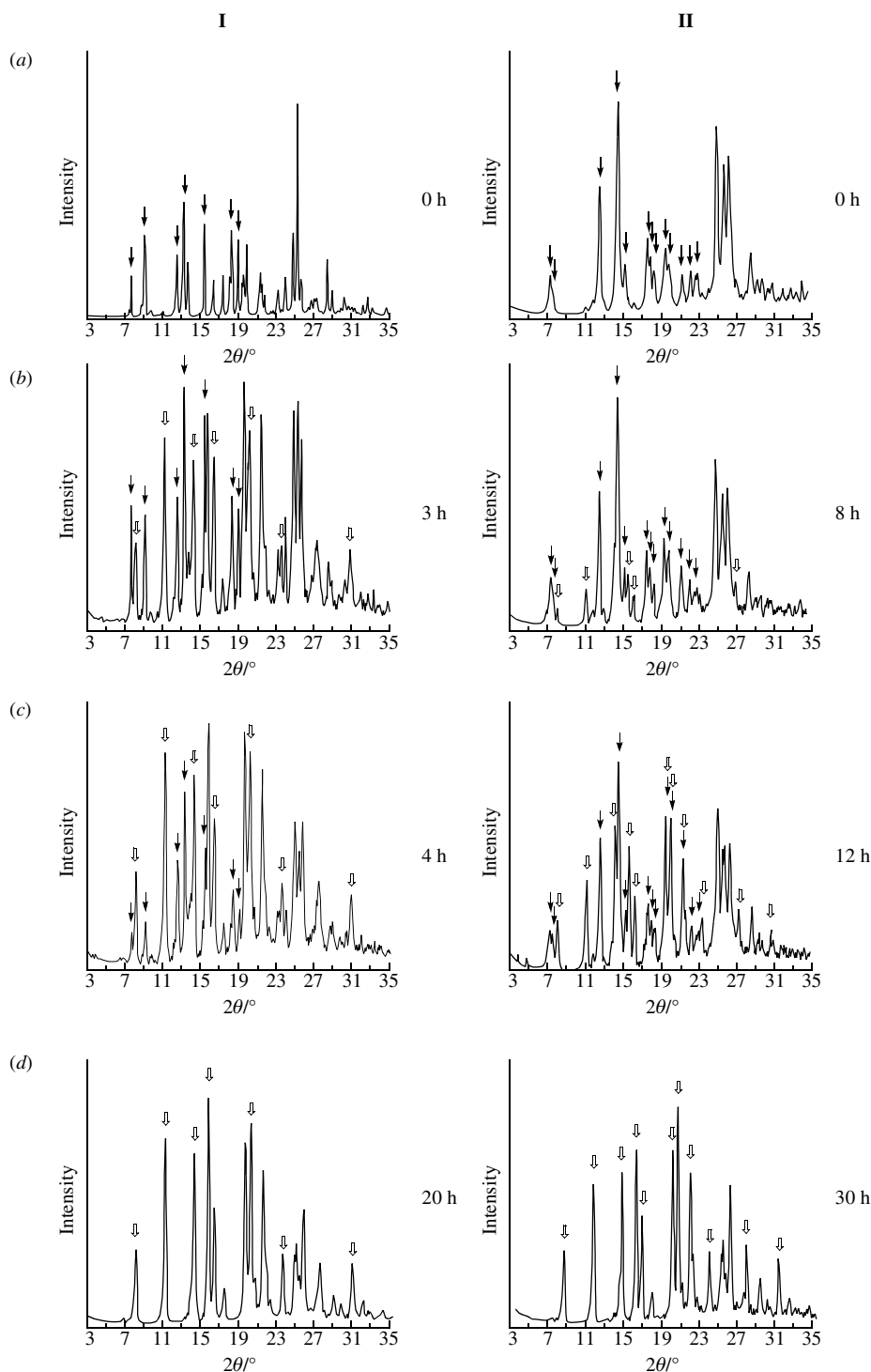
Figure 1 Time-course X-ray powder diffraction patterns of crystals I and II during the colour change at the initial (a), intermediate (b) and (c) and the final (d) stages.
